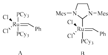
Figure 1. Ruthenium-based olefin metathesis catalysts.
