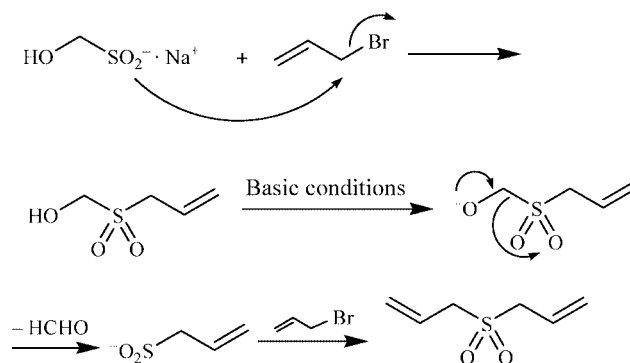
Scheme 2. Proposed mechanism for the formation of sulfone derivatives.
