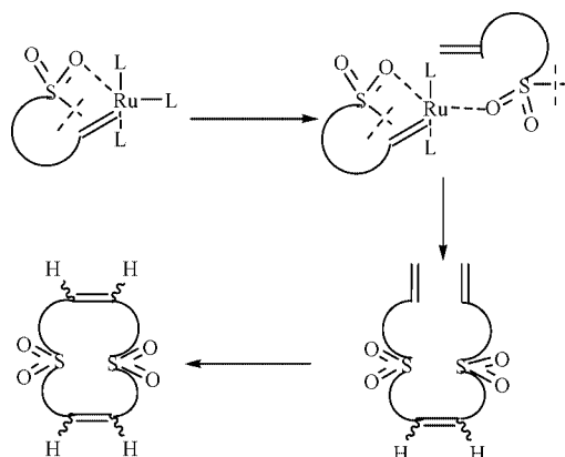
Figure 2. Possible mechanism for the formation of sulfone dimers.
